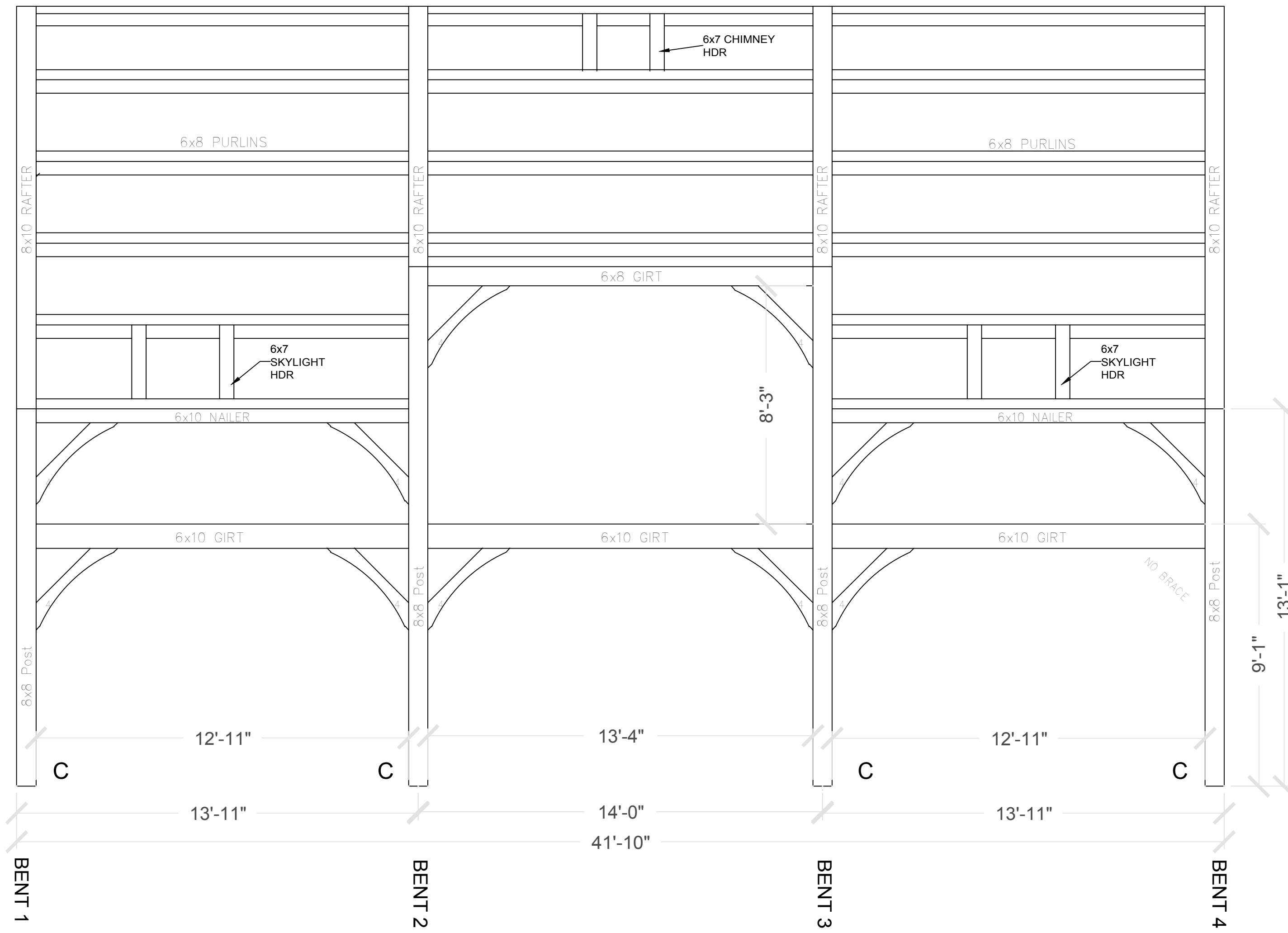
FRAME ELEVATION SCALE 3/8" = 1'
