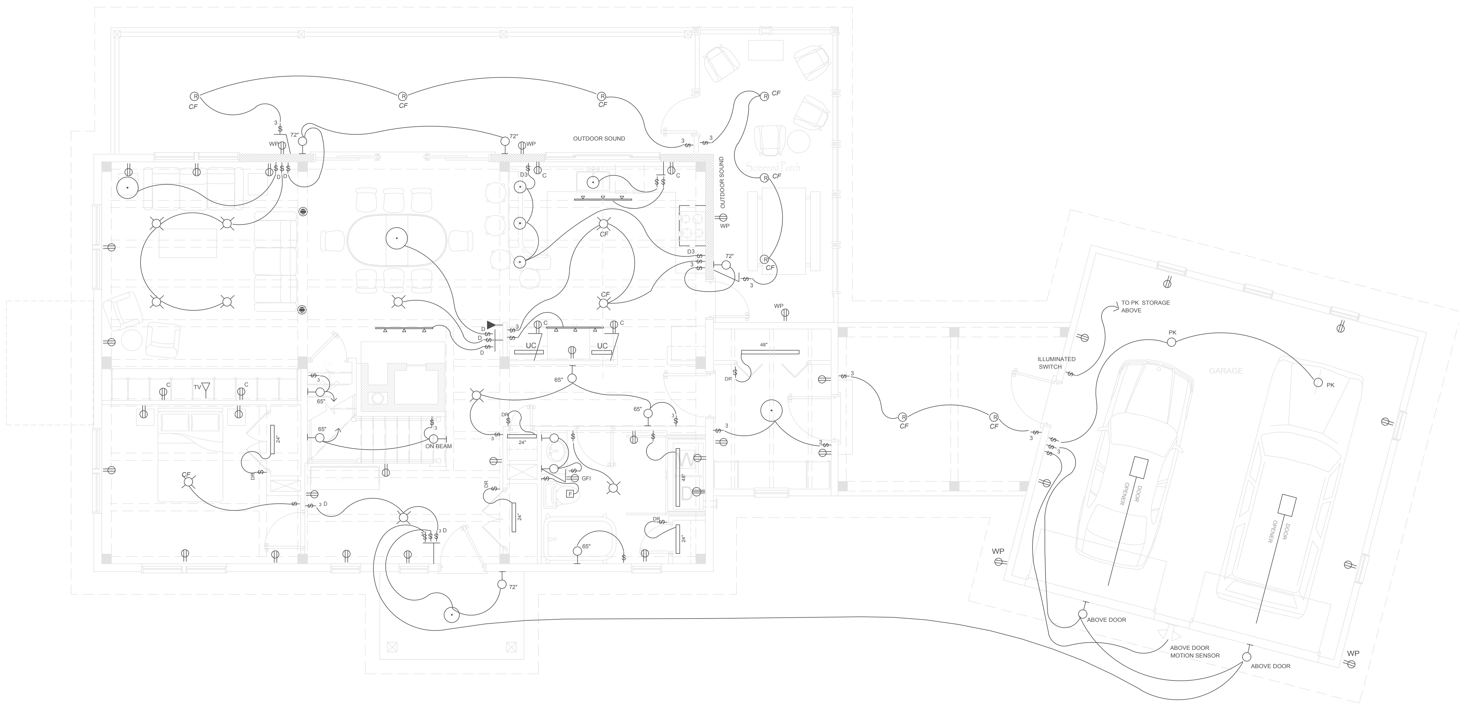
MAIN FLOOR ELECTRICAL PLAN
