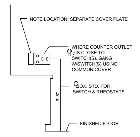
MULTIPLE ELECTRICAL OUTLETS NEAR COUNTER
